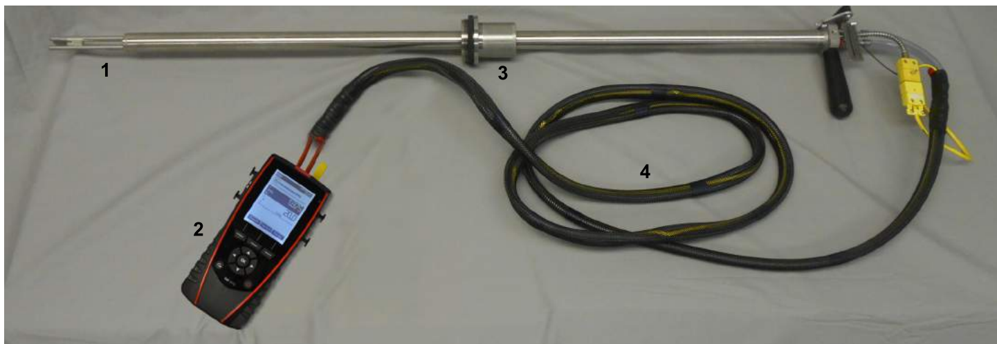
Velocity testing in a coal piping system
