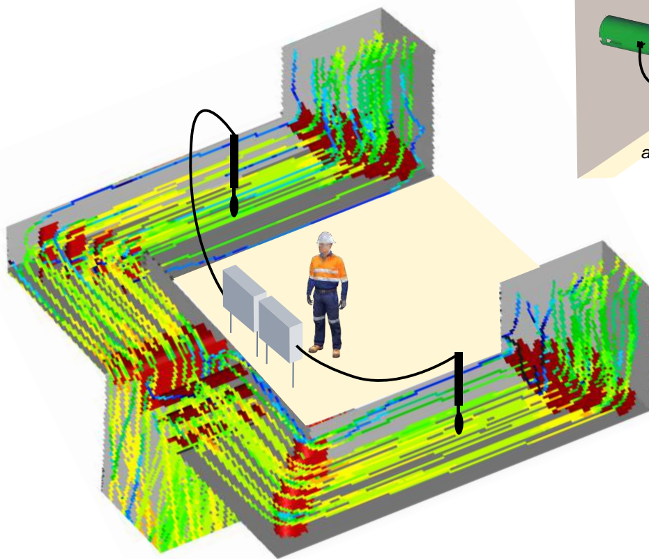
Airflow Guardian measures combustion air with DAP probe in a branching duct system
