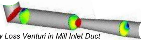
Low Loss Venturi in Mill Inlet Duct
